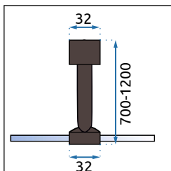
2. Bracket
