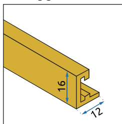
2. Sliding guide
