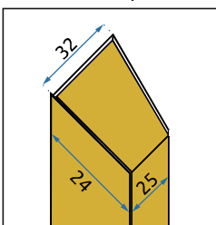
1. Wall adapter
