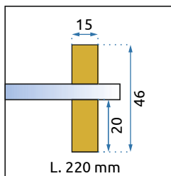
3. Handle
